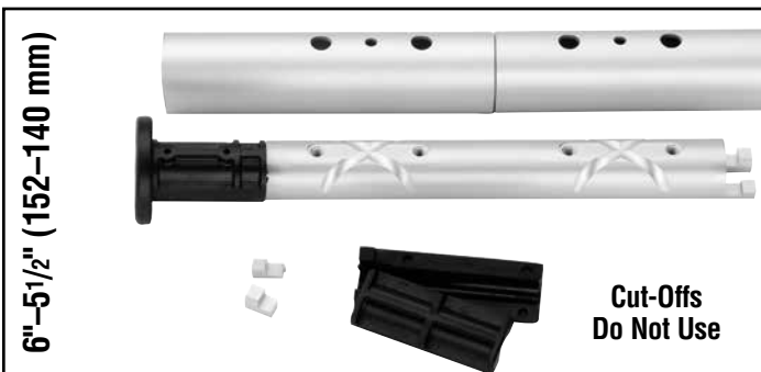
6" - 5 1 / 2 " (152-140 mm) Do not use plastic bushing above top connector. Shorten top of connector and if necessary shorten trim cap.
